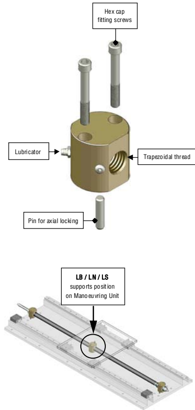
LB/LN/LS supports - exploded diagram
